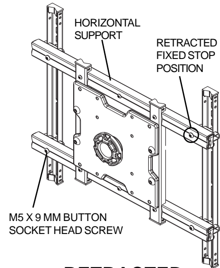
RETRACTED POSITION
