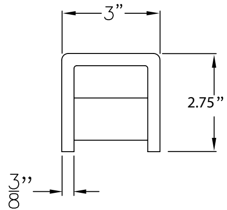
4X DETAIL END OF THRESHOLD
